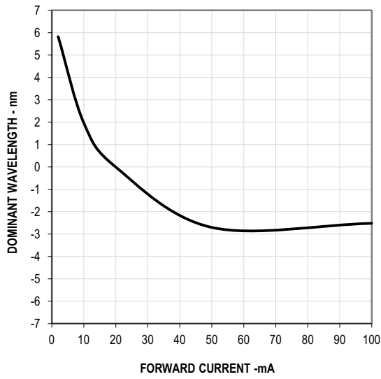
Figure 6: Wavelength vs. Forward Current
