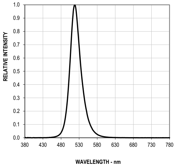
Figure 2: Intensity vs. Wavelength
