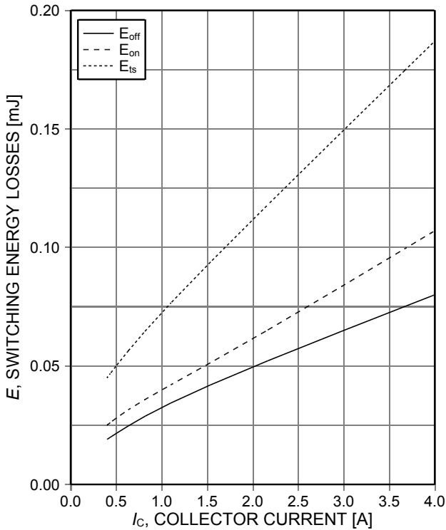
Figure 13. Typical switching energy losses as a function of collector current (inductive load, T_{vj}=175^{\circ}\text{C} , V_{CE}=400\text{V} , V_{GE}=15/0\text{V} , r_G=43\Omega , Dynamic test circuit in Figure E)
