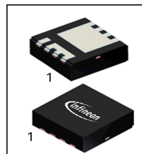
PG-TSDSON-8-33
