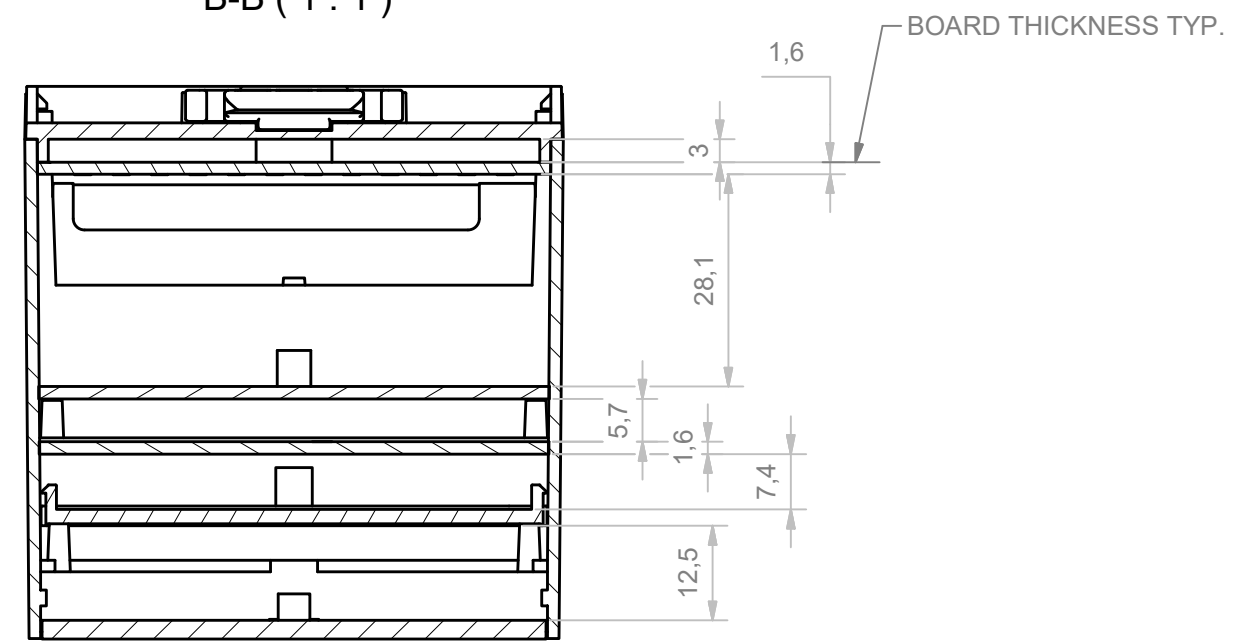
B-B (1:1)
