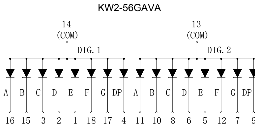
Internal Circuit Diagram (Common Anode)
