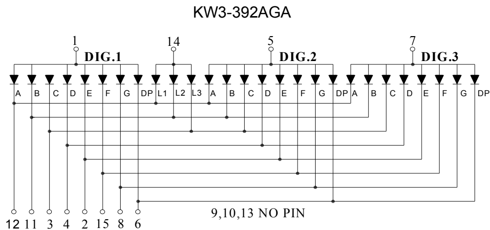
Internal Circuit Diagram (Common Anode)
