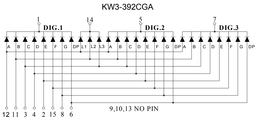
Internal Circuit Diagram (Common Cathode)
