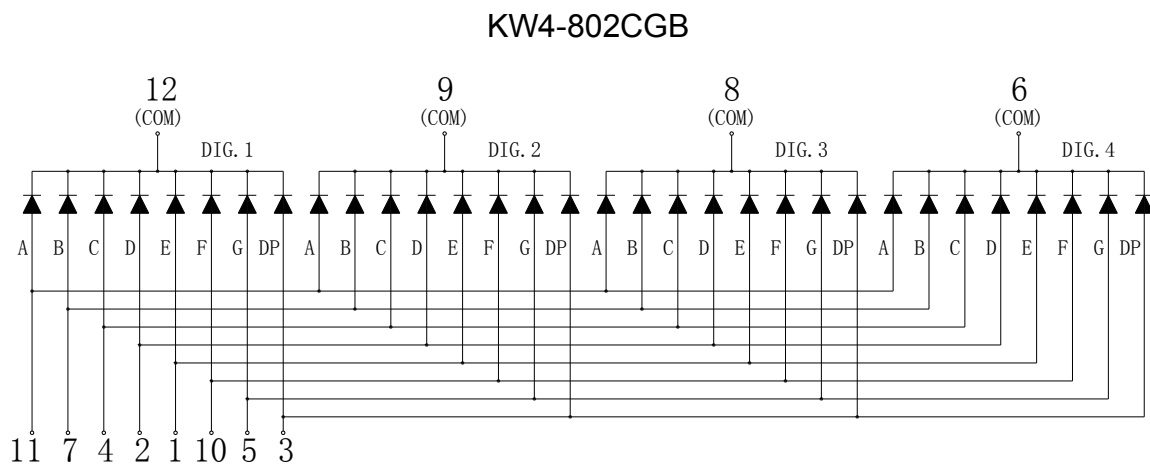
Internal Circuit Diagram (Common Cathode)
