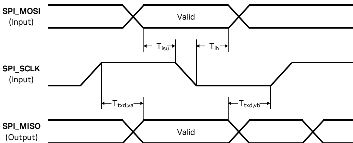
Figure 12: SPI_MOSI, SPI_MISO, SPI_SCLK timings
