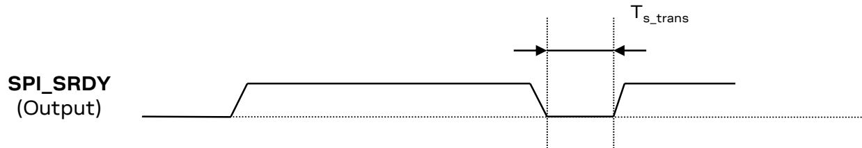
Figure 14: SPI_SRDY transition
