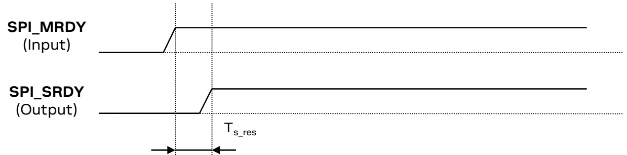
Figure 15: SPI_SRDY response
