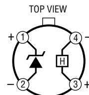
H PACKAGE 4-LEAD TO-46 METAL CAN INSIDE THERMAL SHIELD
