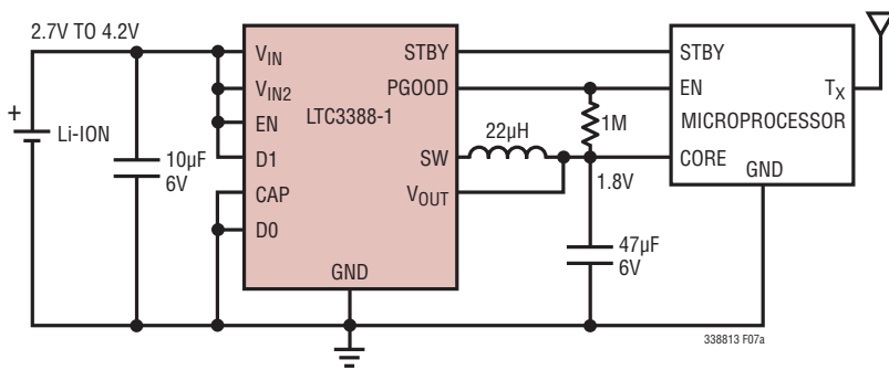
Figure 7. 1.8V Step-Down Converter Powering a Microprocessor with a Wireless Transmitter and 45mA Load Step Response
