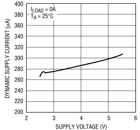
Dynamic Supply Current vs Supply Voltage
