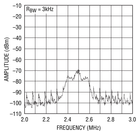
Figure 1b. Output Noise Spectrum of the LTC3543 Spread Spectrum Buck Switching Converter. Note the Reduction in Fundamental and Harmonic Peak Spectral Amplitude Compared to Figure 1a.
