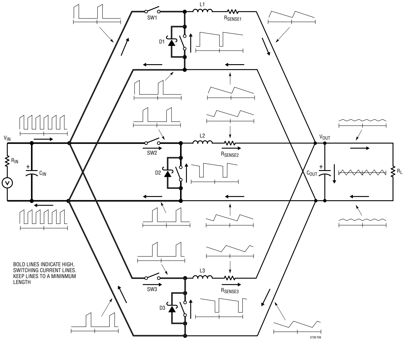
Figure 9. Branch Current Waveforms
