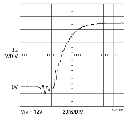
BG Turn-On Waveform Driving Renesas RJK0301
