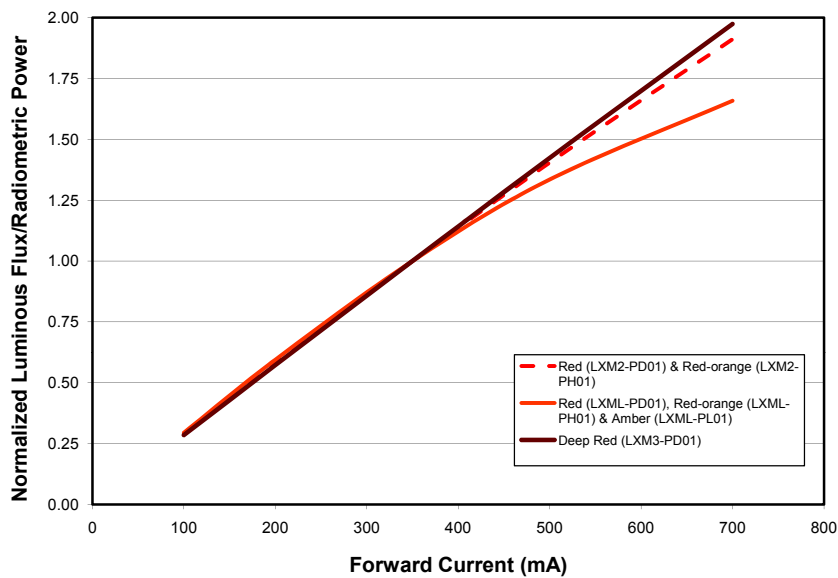
Figure 13. Relative luminous flux vs. forward current for red, deep red, red-orange and amber at Thermal Pad = 25°C maintained.
