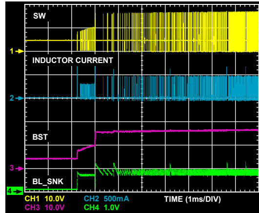
Figure 12. Boost Startup
