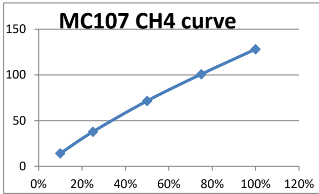
Fig3.Sensitivity Curve
