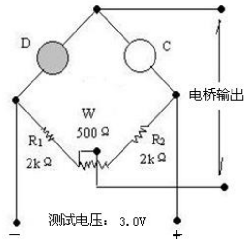
Fig2. Basic Test Circuit
