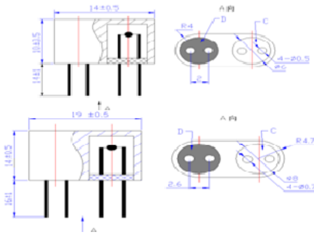
Fig1. Sensor Structure
