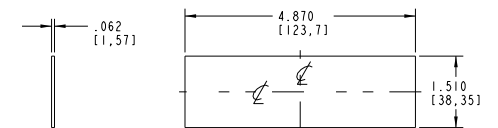
REAR PANEL
