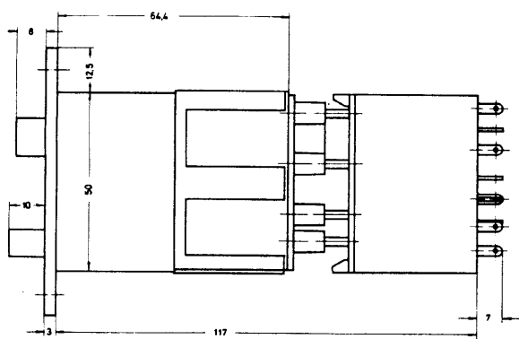
FR 319 Cutout 51,0 x 51,0 mm
