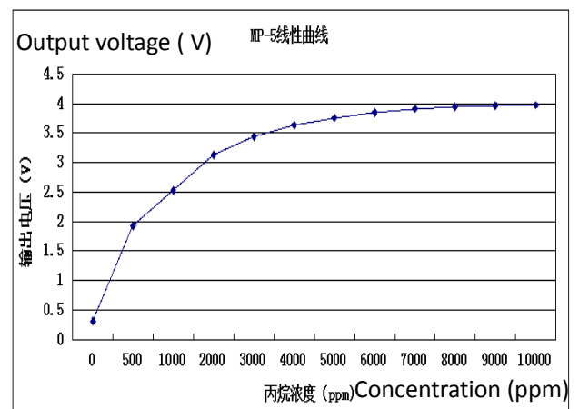
Fig6. Linearity curve
