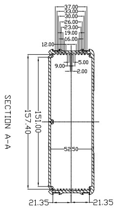
ENCLOSURE PROFILE
