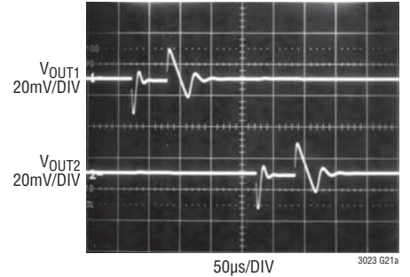
Channel-to-Channel Isolation
