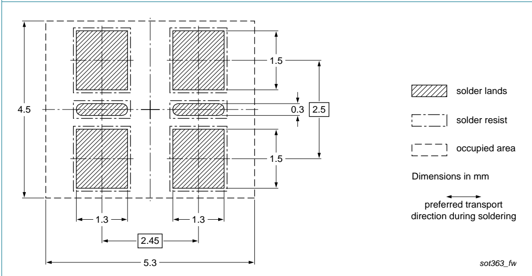
Fig 14. Wave soldering footprint PUMB1 (SOT363)
