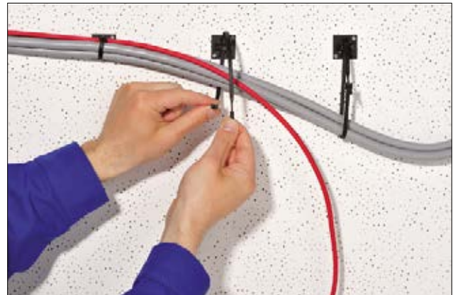
Without additional effort only Q-ties can be used for temporary and final cable bundling.
