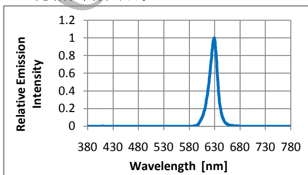
Fig.7- Spectrum Distribution
