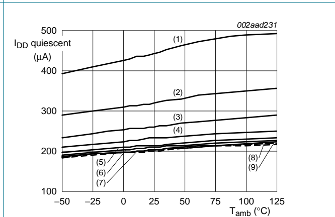
Conversion rate: (1) 16 Hz (2) 8.0 Hz (3) 4.0 Hz (4) 2.0 Hz (5) 1.0 Hz (6) 0.5 Hz (7) 0.25 Hz (8) 0.12 Hz (9) 0.06 Hz Fig 16. Typical I DD quiescent current versus temperature and conversion rate (V DD = 3.3 V)
