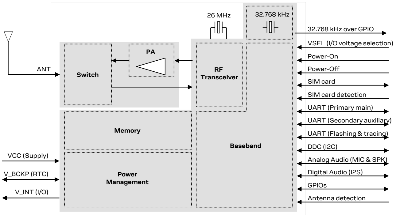
Figure 1: SARA-G450 modules' block diagram
