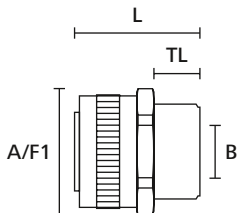
HeloGuard fitting, straight with fixed external thread
