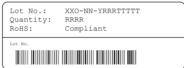
Figure 20: First label on reel: XX = Sensor Type (25 for SHT25), O = Output mode (D = Digital), NN = product revision no., Y = last digit of year, RRR = number of sensors on reel divided by 10 (200 for 2000 units), TTTTT = Traceability Code.
