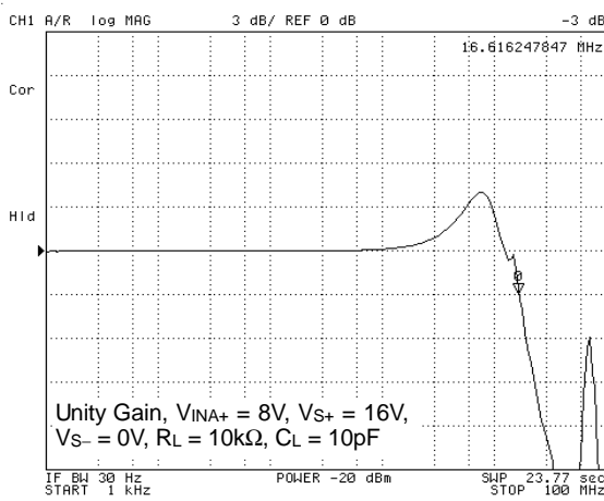
-3dB Bandwidth
