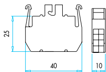
B Serisi Ampul Takılabilen Işıklı Blok Neon Lamp Mountable B Series Light Block
