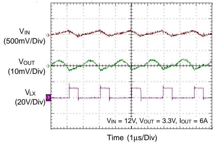
Voltage Ripple
