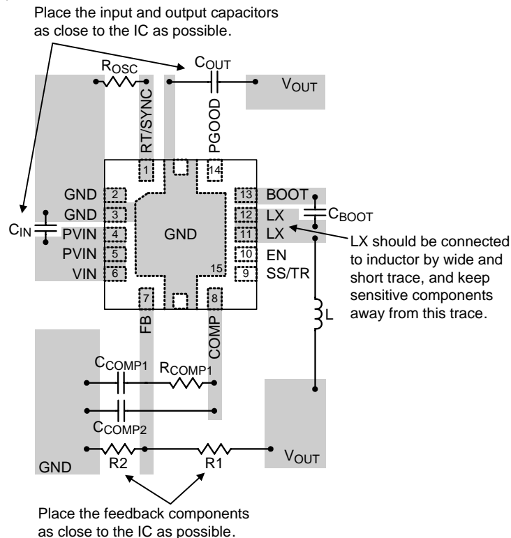
Figure 11. PCB Layout Guide
