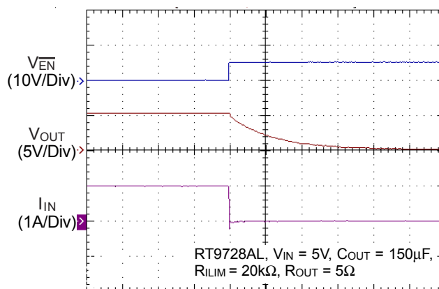
Time (500µs/Div)
