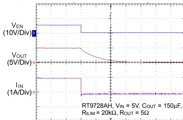
Time (500µs/Div)
