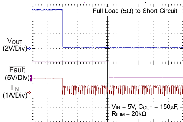
Time (2.5ms/Div)
