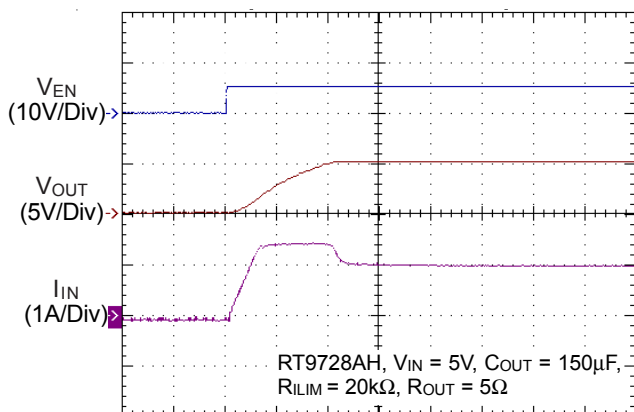
Time (500µs/Div)
