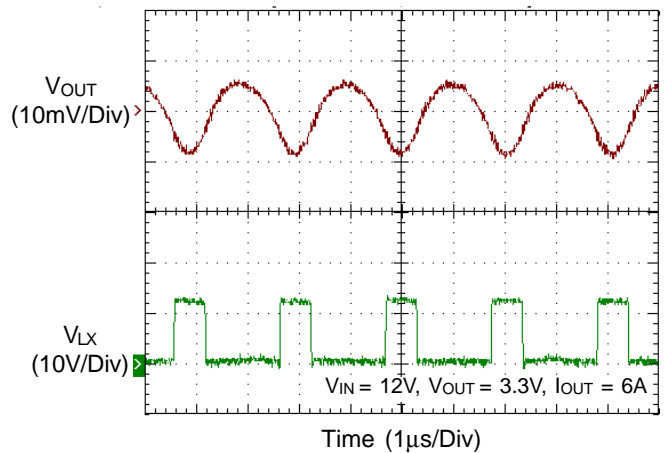
Voltage Ripple
