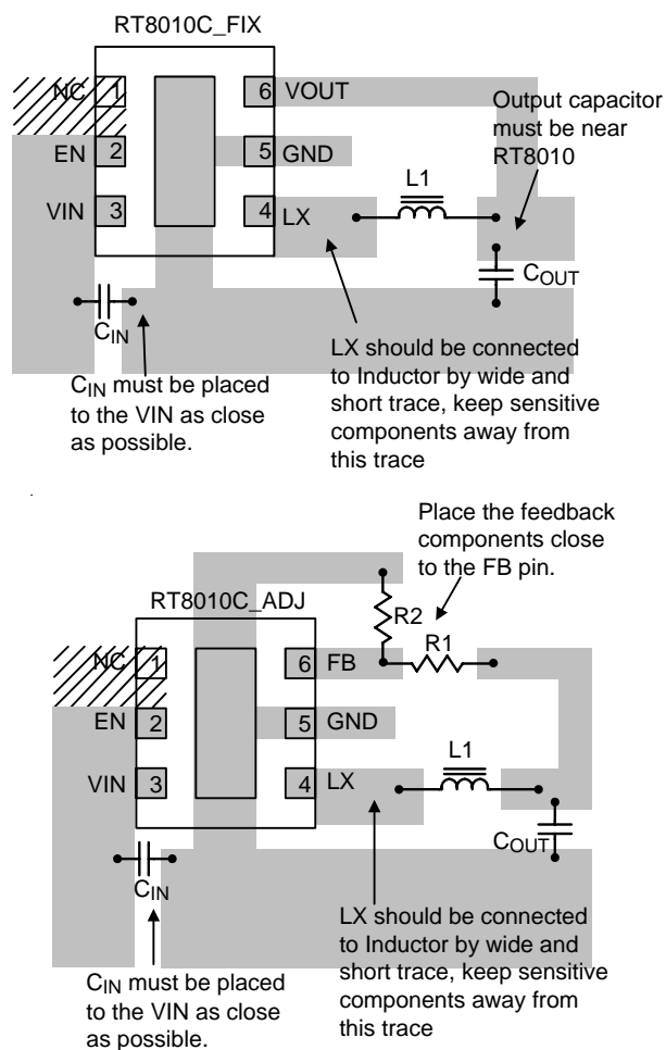
Figure 6. PCB Layout Guide
