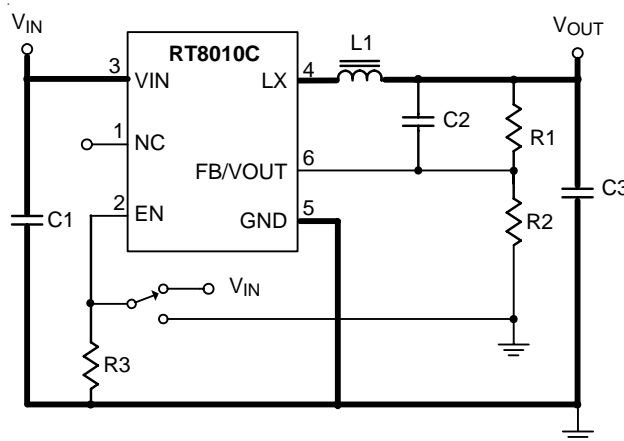
Figure 5. EVB Schematic
