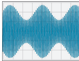
Amplitude modulation
