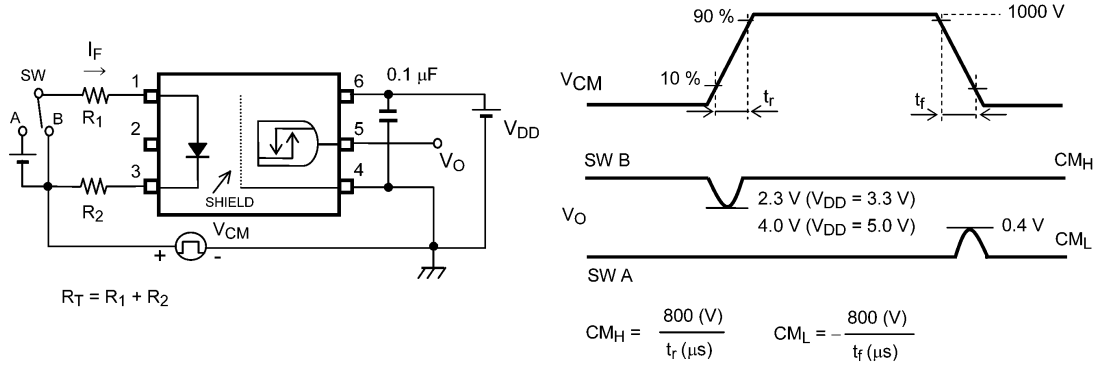
Fig. 12.1.7 Common-Mode Transient Immunity Test Circuit and Waveform
