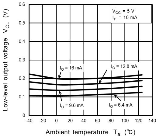
Fig. 13.2.3 V OL - T a
