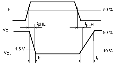
Fig. 12.1.5 Switching Time Test Circuit and Waveform
