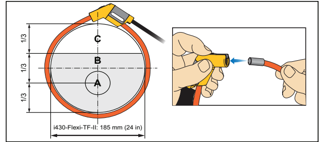
Figure 1. Connecting the flexible probe around the conductor.
