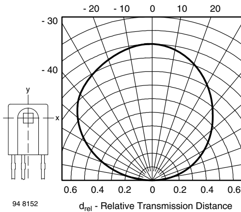
Fig. 5 - Vertical Directivity \phi_y
