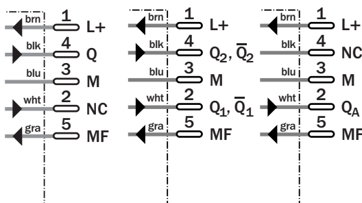
5-pin, M12 5-pin, M12 5-pin, M12
