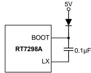
Figure 9. External Bootstrap Diode
