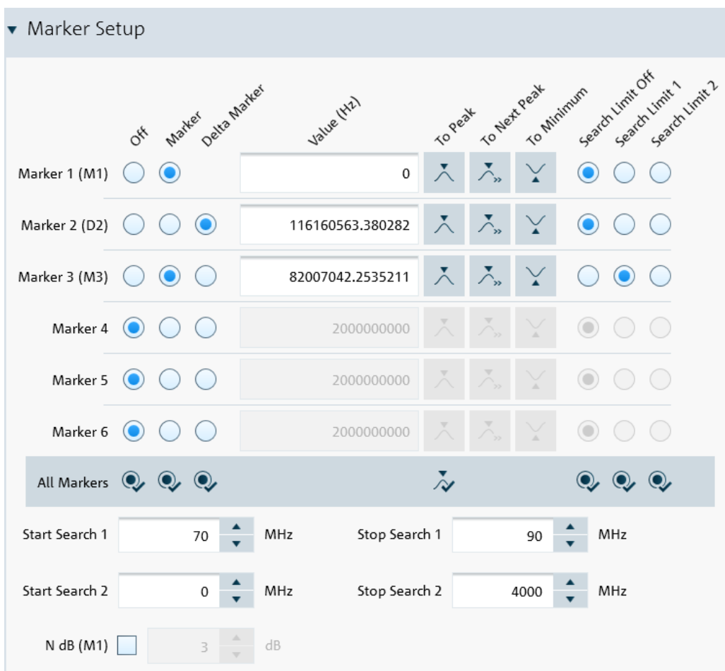
Figure 4-6: Marker setup
