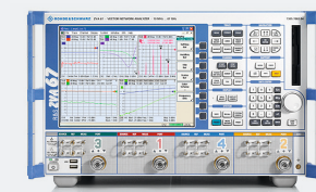
R&S®ZVA Network Analyzer
