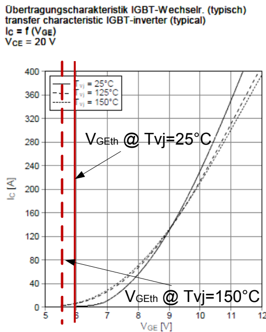
Figure 10: Typical transfer characteristic
