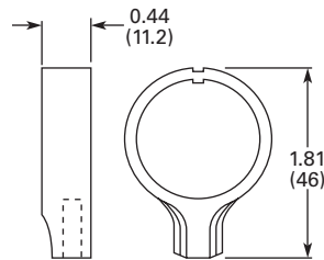
Lever for Roto-Push Operator Catalogue No. 10250TA13
