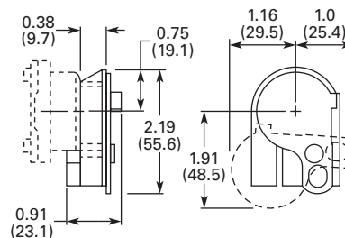
Padlock Attachment for Maintained Push-Pull Operator Catalogue No. 10250TA64
