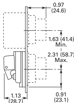
Maintained Contact Attachment Catalogue No. 10250TA17 Typical
