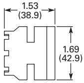
Protecting Shroud for Mushroom Head Button Catalogue No. 10250TA6
