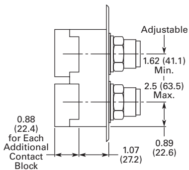
Maintained Pushbutton Catalogue No. 10250TA66 Typical
