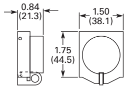
Padlock Hasp or Flip-Up Guard Catalogue No. 10250TA38
