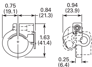
Padlock Attachment—For Extended Pushbutton Catalogue No. 10250TA26
