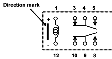
Non-latch type (Not energized position)
