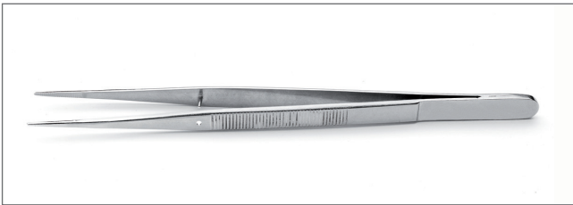
648.SA Serrated handles. Tips: straight, strong, fine, line serrated. OAL: 155mm
