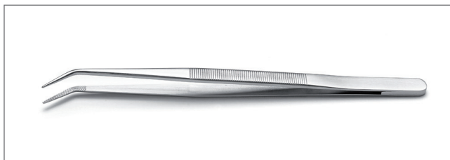
124.SA Serrated handles. Tips: fine, bent, rhomb serrated. OAL: 150mm
