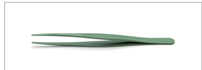
321.SA.T Teflon coated. Serrated handles. Tips: straight, rounded, flat. OAL: 120mm
